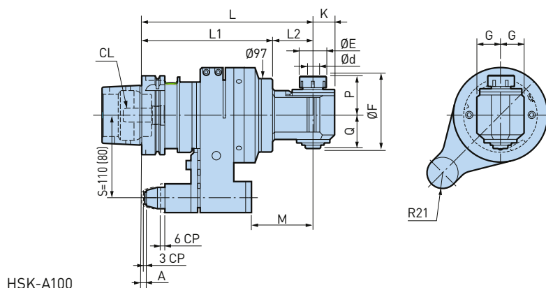
HSK-A100
