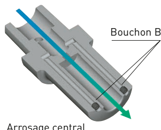
Arrosage central
