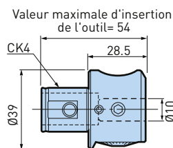
Tête EWN2-22CK4 Stroke 0 - 2mm
