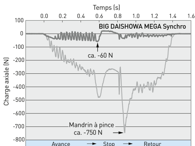
Pince
